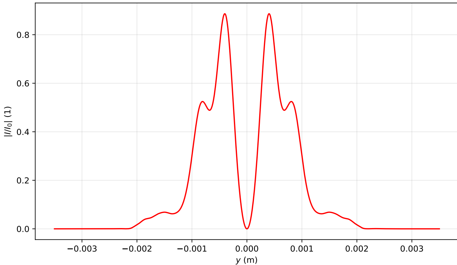
Intensity profile I(x=0, y, z=1.831)/I_0 , \text{Pin}=6.0\text{Pcr} , artificial time
